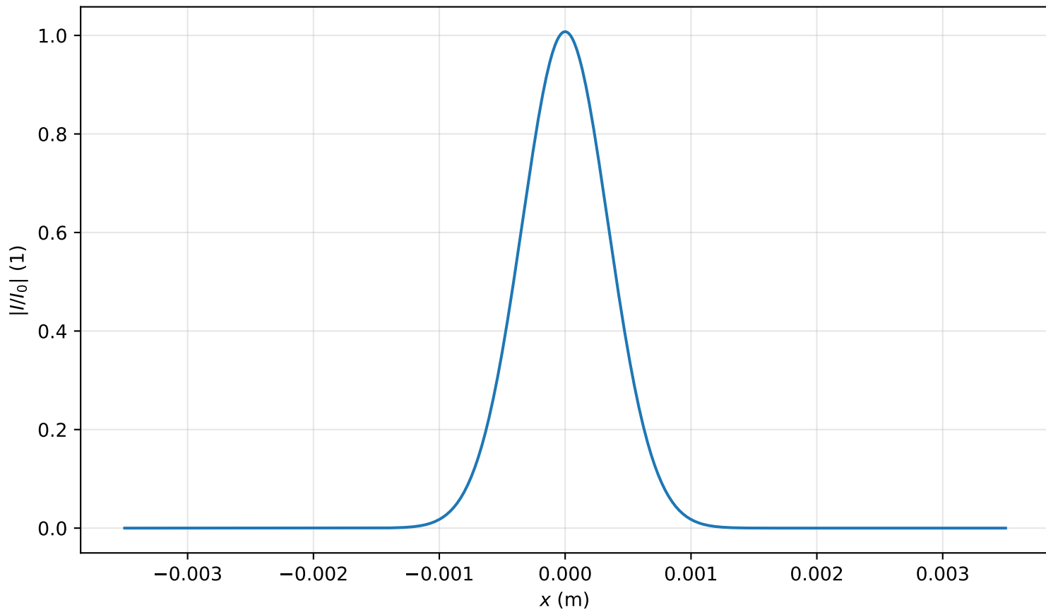
Intensity profile I(x, y = 0, z = 0.239m)/I_0 , P_{in}=0.4P_{cr} , artificial time
